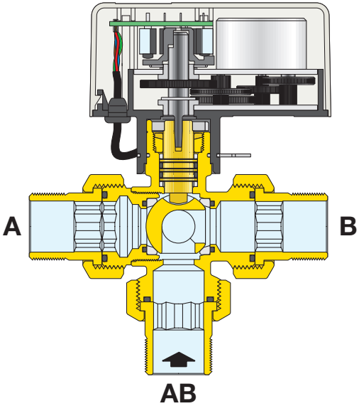
3-way 6443.. code, diverter version
