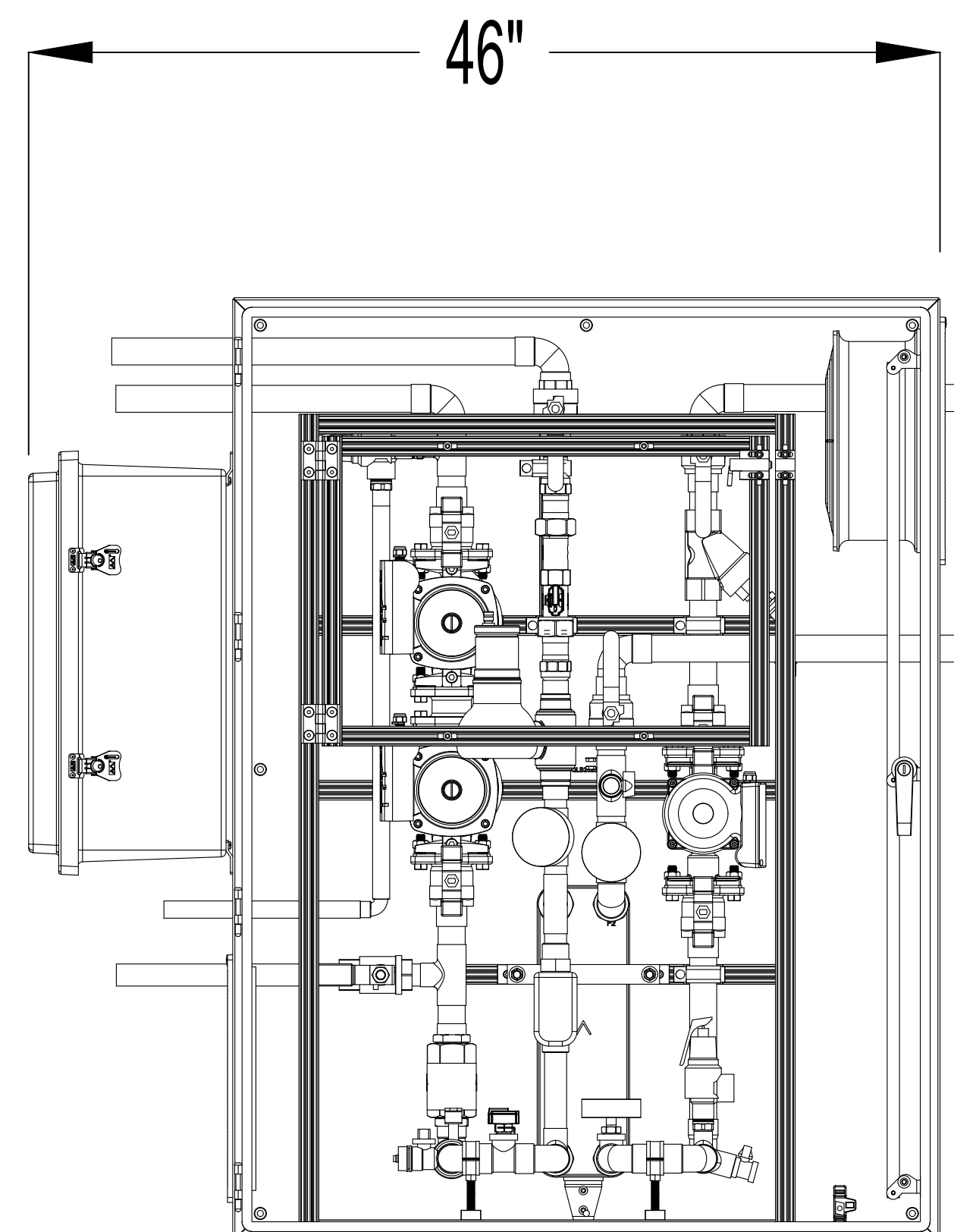
SETO-1020-13-50-E1 (without door to show internal components)
